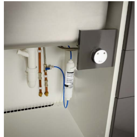
Under the sink (inside the base unit)
