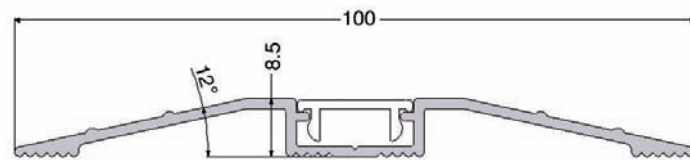
Threshold kit side profile
