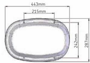
50mm Plinth
