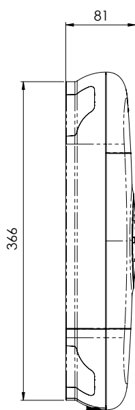
Dimensions (mm)
