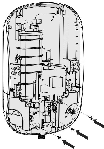
Fasten the screws holding the outlet connector and bottom cover
