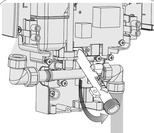
Pull the outlet connector up
