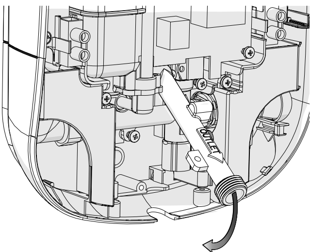
Carefully push the outlet connector down to its home position
