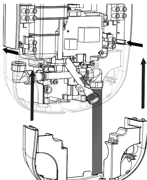
Slide back in the bottom cover plate
