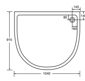
U Shape Quadrant
