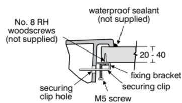
section through basin showing securing clip
