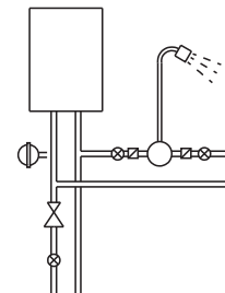
Instantaneous heated system (Gas or Electric)
