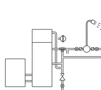
Mains pressurised hot water system
