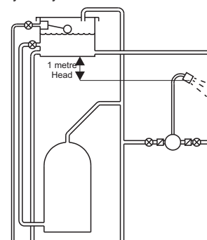
Gravity fed system
