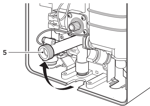
Outlet connection 5
