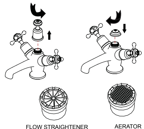
FLOW STRAIGHTENER
