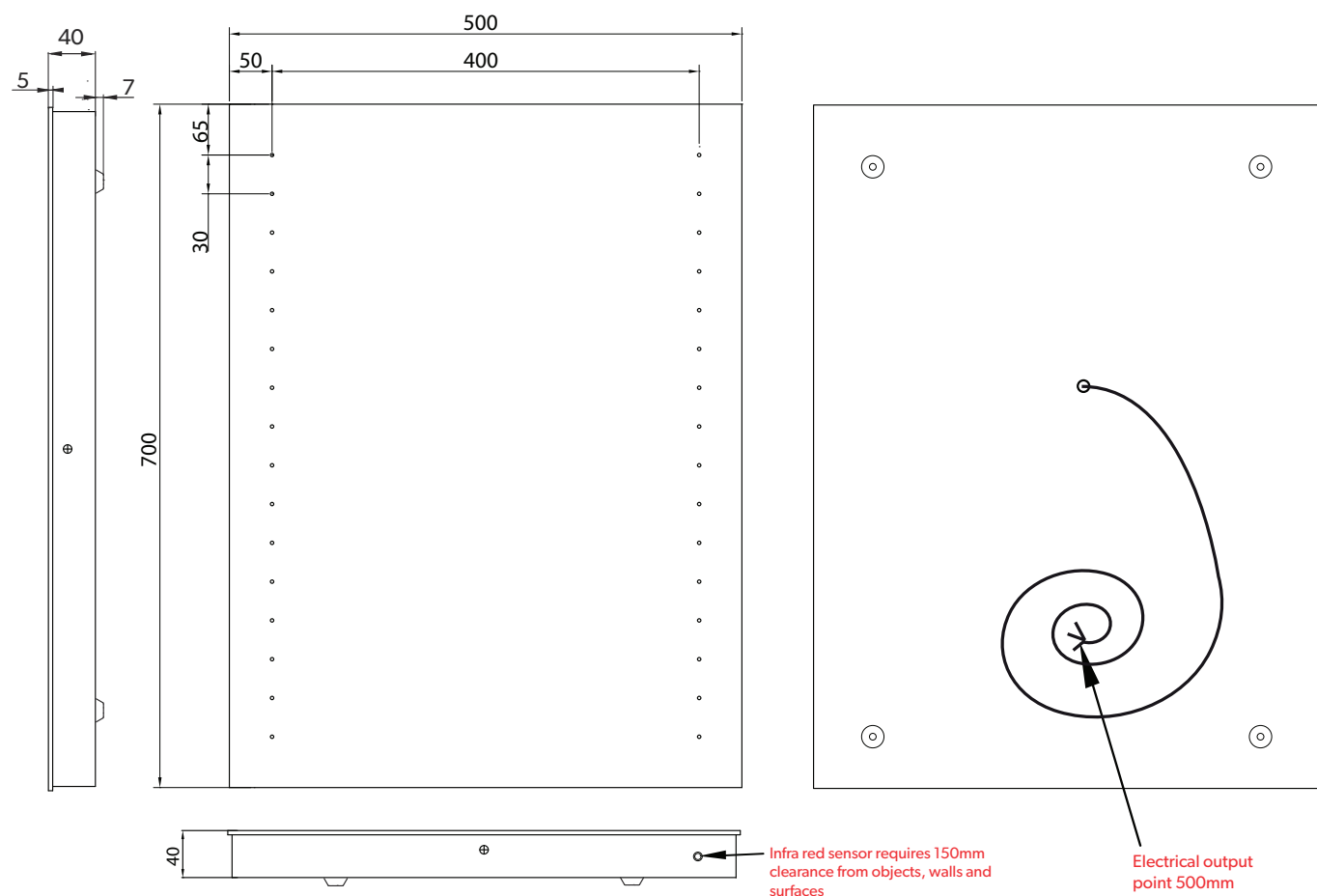
Front View
