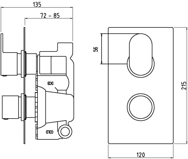
1/2" BSP CONNECTIONS
