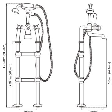
Freestanding Mixer Taps, With Standpipes, Ceramic Disc Valve
