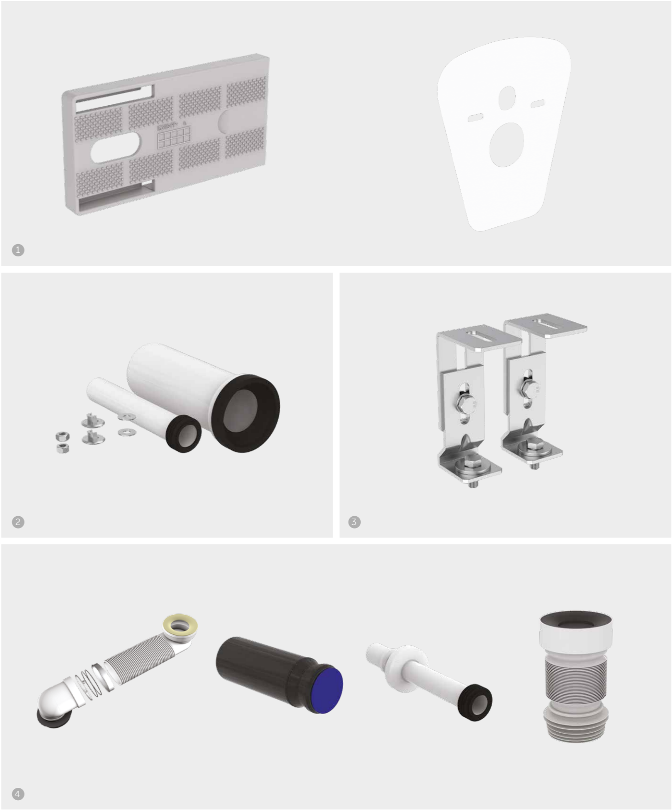
1. Noise insulation kits: Frame to floor; WC 2. Extended bowl fixing kit 3. Corner installation kit 4. S-bend outlet; horizontal outlet WC; telescopic connection pipe; flexible outlet WC bend
