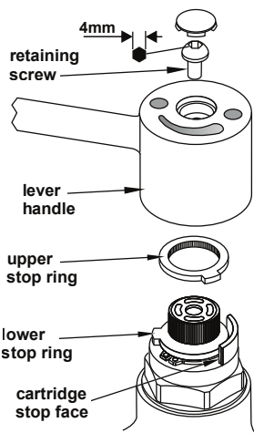
Figure 10.1 Adjusting the pre-set temperature
