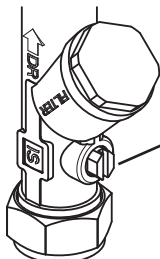
Fig 6.4 Isolating screw
