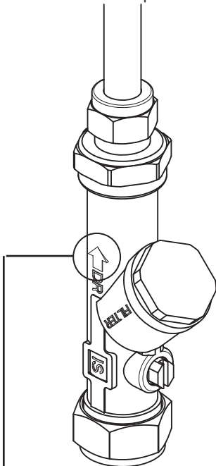
Fig 6.3 Fitting copper pipe
