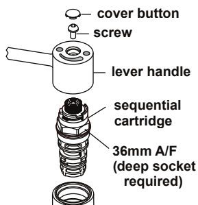
Figure 10.2 Exploded view showing sequential cartridge
