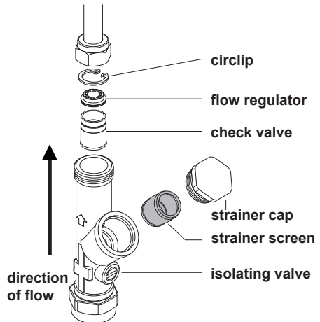
Fig.11.2 Exploded view of isolating valve
