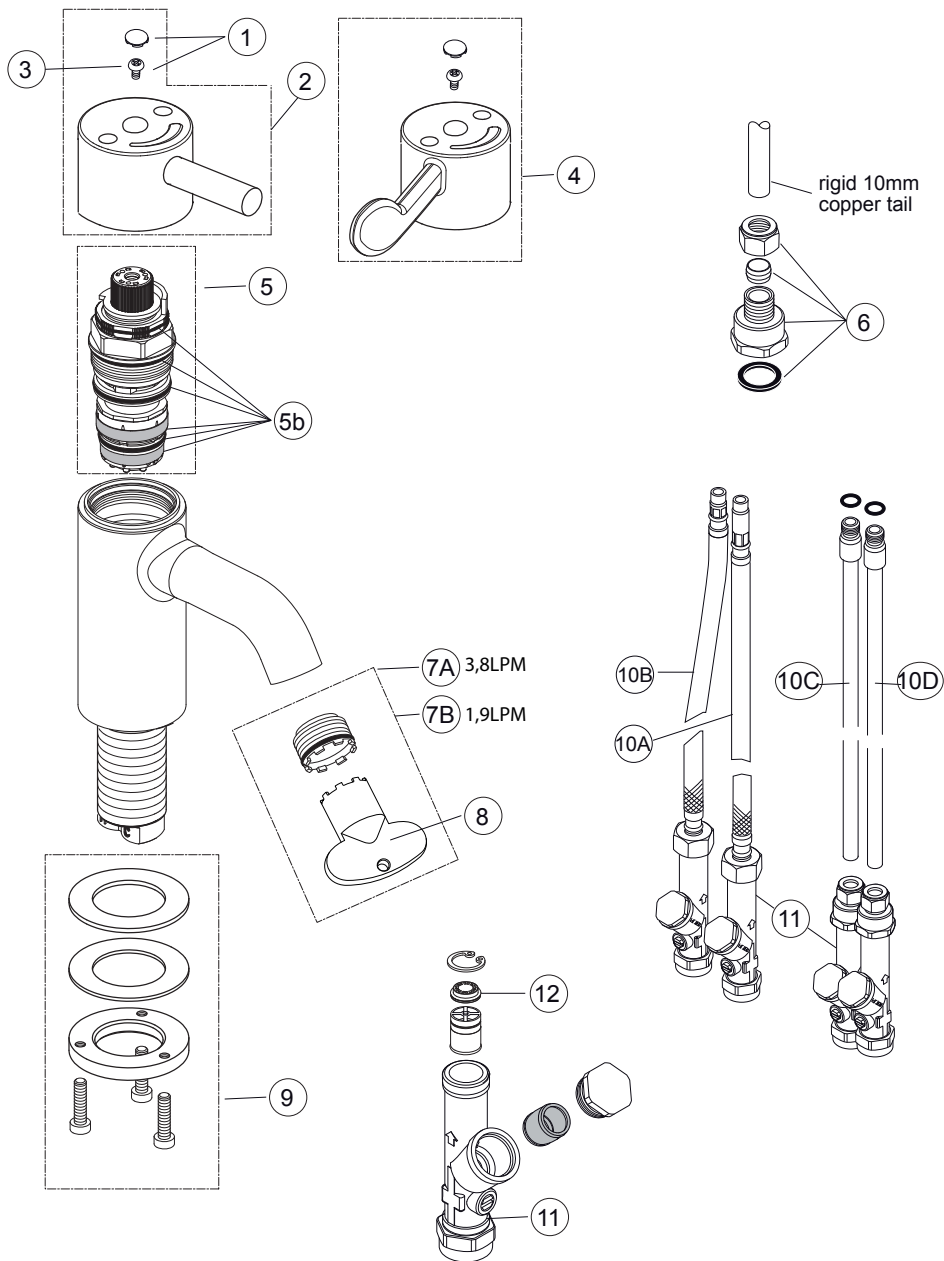
Fig.13 Exploded views
