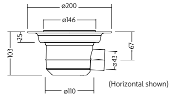
Vinyl Floor Gully - Horizontal Outlet Code: UTVCO1/H (CHROME) Price: £126.95 Exc. VAT £152.34 Inc. VAT* Code: UTVG01/H (GREY) Price: £0.00 Exc. VAT £0.00 Inc. VAT*
