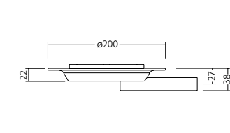
Tiled Floor Gully - For Pumped Waste Code: DSS2 Price: £174.46 Exc. VAT £209.35 Inc. VAT*
