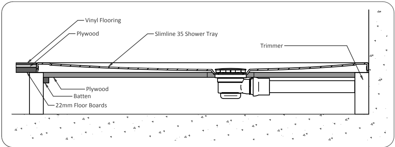
Diagram 1. Cross section of Slimline 35 Shower Tray and joists.
