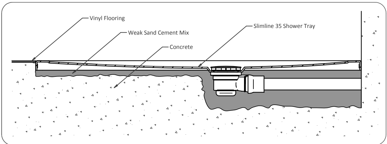
Diagram 2. Cross section of Slimline 35 Shower Tray and concrete floor.
