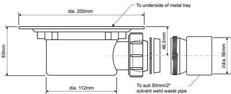
Standard waste option for tiled floors
