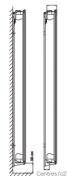
Type 10 Vertical Flat Radiator
