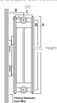
Type 22 Double Convactor
