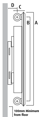
Type 11 Single Convactor
