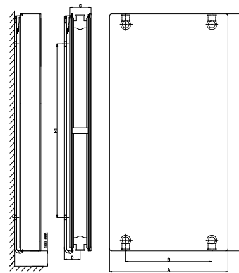
Type 20 Vertical Flat radiator
