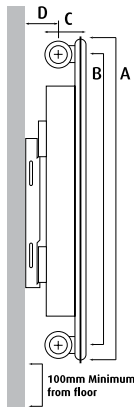
Type 11 Single Convector
