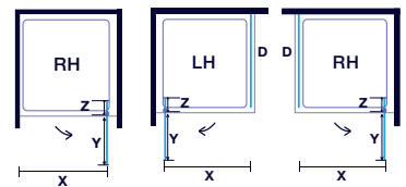
Pivot Door with Side Panel
