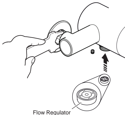
Flow Regulator
