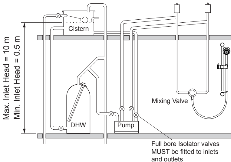
System Layout for Mira Twin Ended Pump
