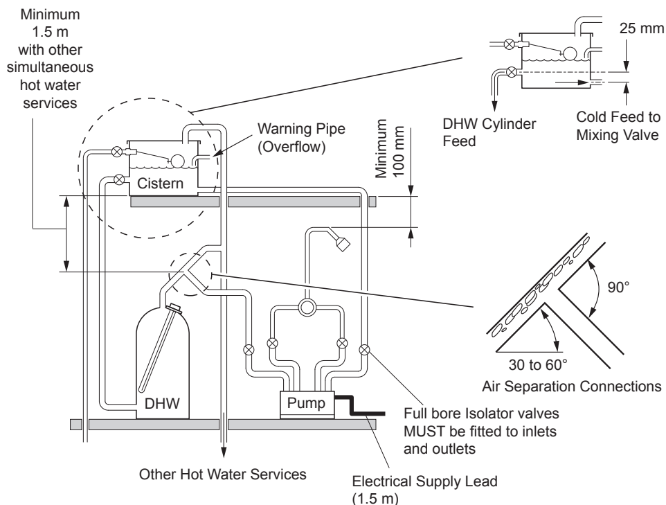
System Layout for Mira Twin Ended Pump Fig. 2
