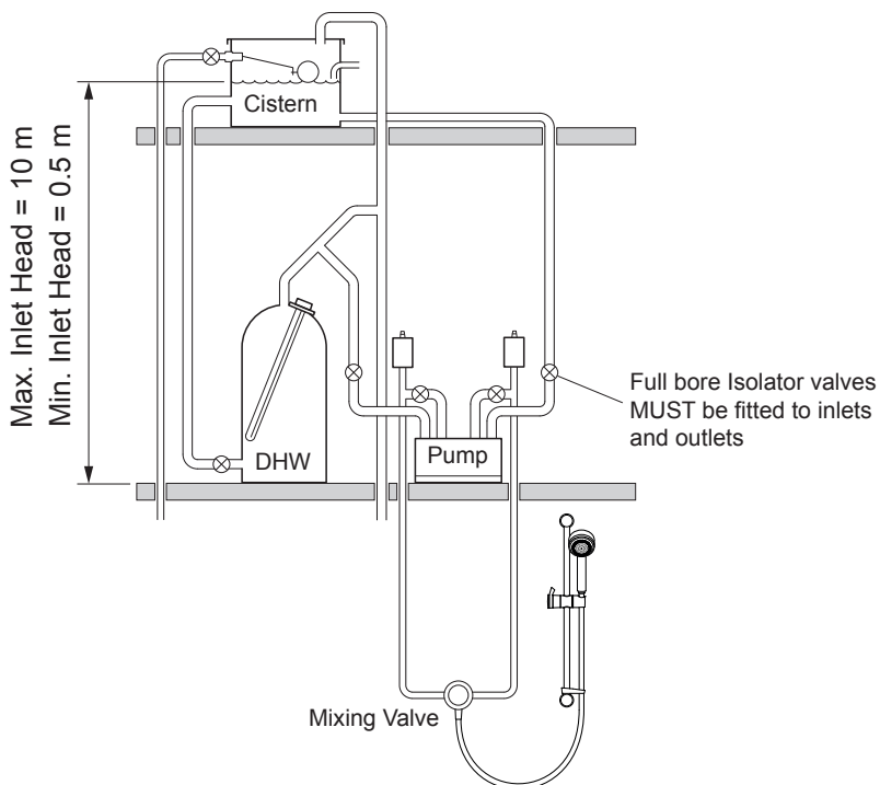
System Layout for Mira Twin Ended Pump
