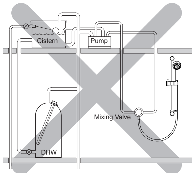
Unsuitable Layout for Mira Enduro Pump
