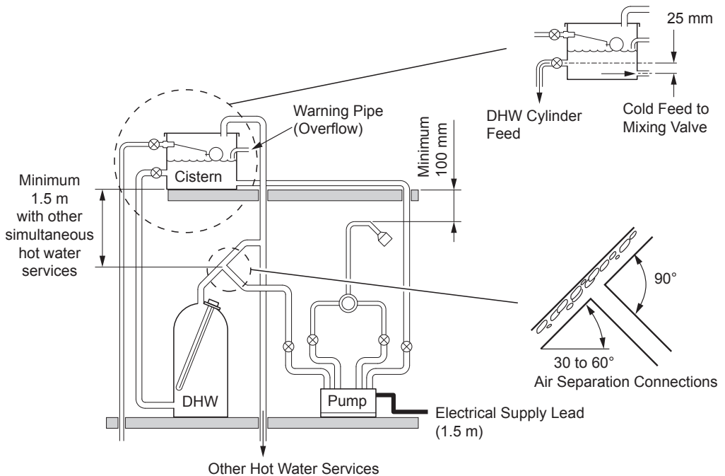
System Layout for Mira Shower Pump Fig. 2
