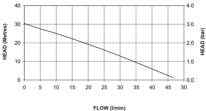
Mira 3.0 bar Brass Twin Ended Pump Performance Graph
