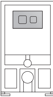
Mid-Height Dual Flush Concealed WC Cistern with Wall Hung Frame H890-1090 x W520mm Flush Plate with Square Buttons ● Chrome XTY007S £406.00 ● White XTY107S £409.00 ● Black XTY407S £423.00 ● Brass XTY807S £456.00
