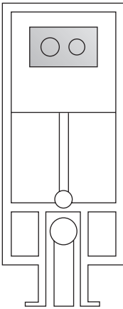
Dual Flush Concealed WC Cistern with Wall Hung Frame H1136-1336 x W520mm Flush Plate with Round Buttons ● Chrome XTY007S £406.00 ● White XTY107S £409.00 ● Black XTY407S £423.00 ● Brass XTY807S £456.00
