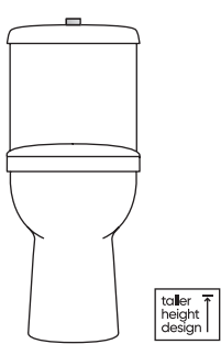
Dual Flush Comfort Height Pan & Cistern Seat included H860 x W380 x D650mm NCS500 £504.00
