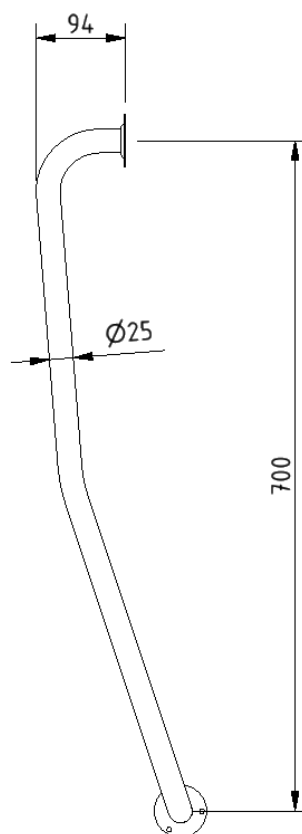
RIGHT-HAND
