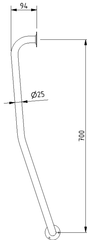
RIGHT-HAND
