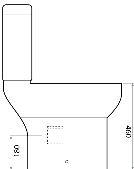
Dimensions (measurements in mm)
