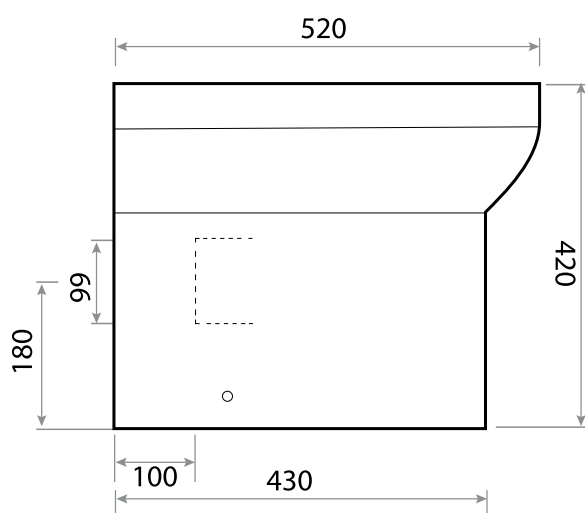
Dimensions (measurements in mm)
