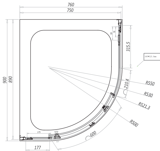
Dimensions (measurements in mm)
