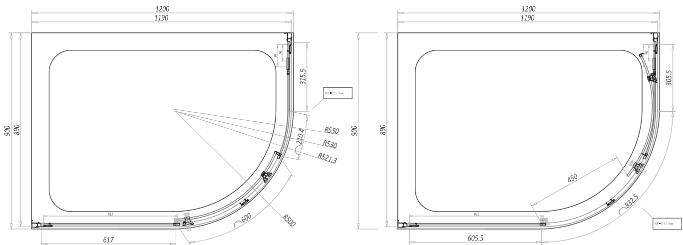
Dimensions (measurements in mm)
