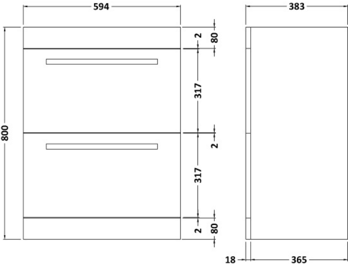
600 FLOOR STANDING 2-DRAWER BASIN UNIT
