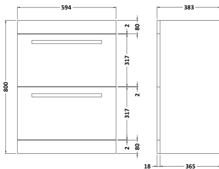
600 FLOOR STANDING 2-DRAWER BASIN UNIT
