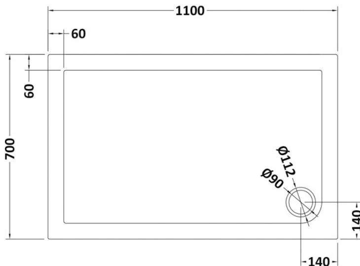
NTP016 - 1100 x 700 RECTANGULAR TRAY
