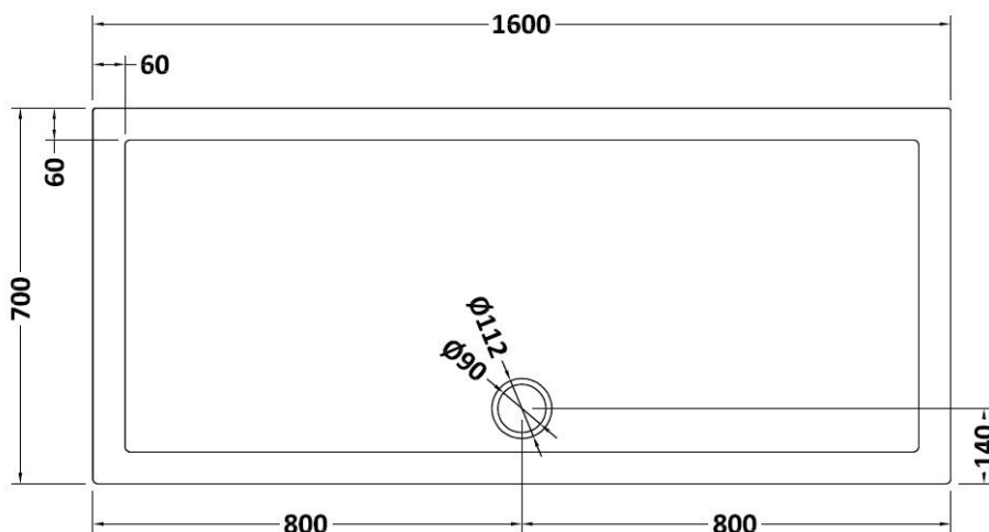
NTP051 - 1600 x 700 RECTANGULAR TRAY
