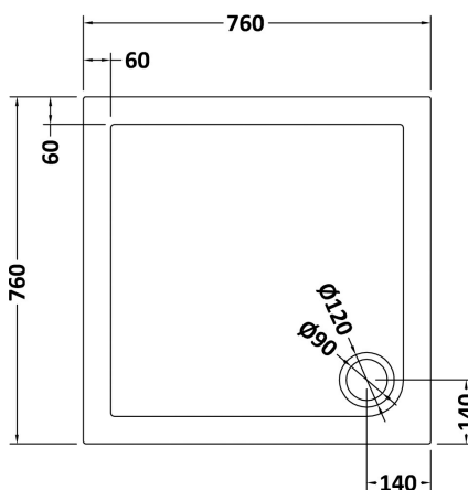
NTP003 - 760 x 760 SQUARE TRAY
