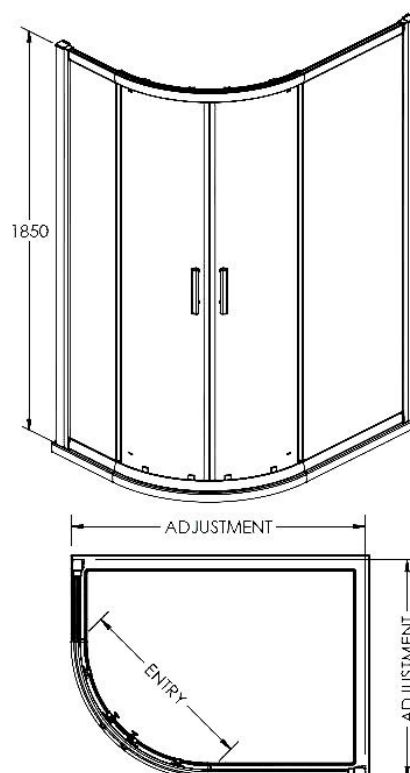
Pacific Offset Quadrant Enclosure
