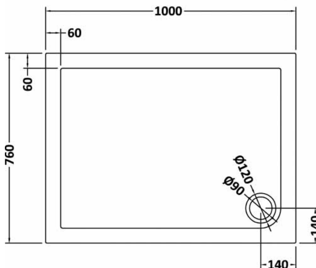
NTP012 - 1000 x 760 RECTANGULAR TRAY
