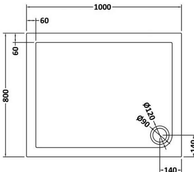
NTP013 - 1000 x 800 RECTANGULAR TRAY
