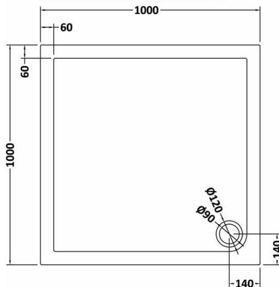
NTP015 - 1000 x 1000 SQUARE TRAY
