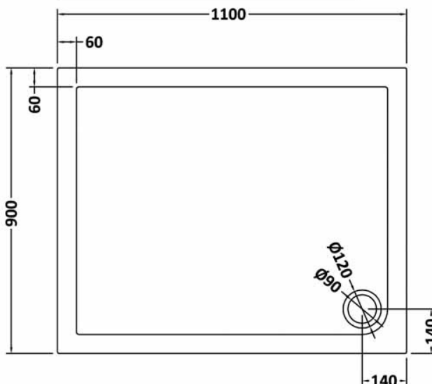
NTP019 - 1100 x 900 RECTANGULAR TRAY
