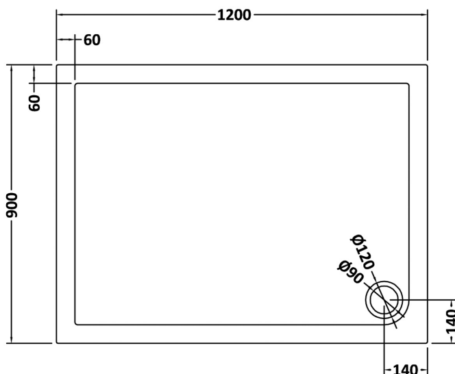
NTP024 - 1200 x 900 RECTANGULAR TRAY
