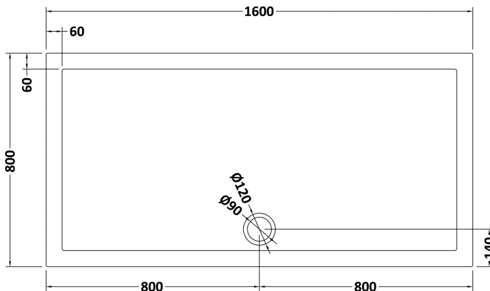
NTP053 - 1600 x 800 RECTANGULAR TRAY
