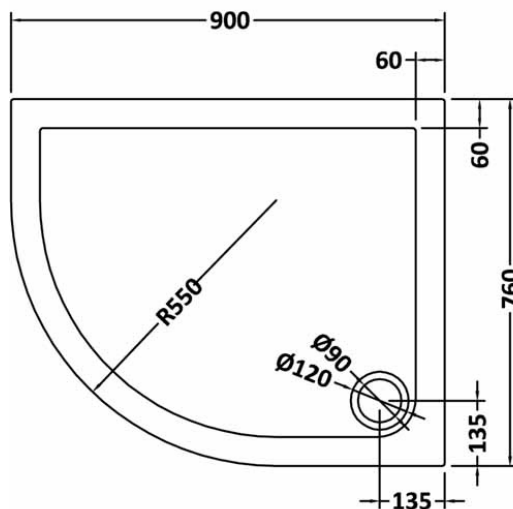
NTP101 - 900 x 760 OFFSET QUADRANT TRAY LH
