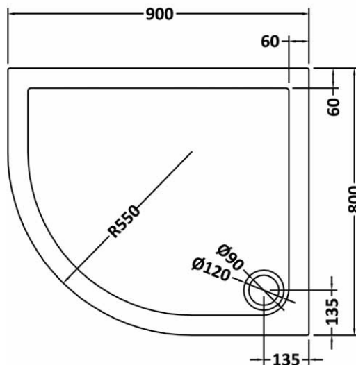
NTP103 - 900 x 800 OFFSET QUADRANT TRAY LH
