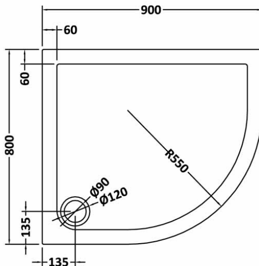
NTP104 - 900 x 800 OFFSET QUADRANT TRAY RH
