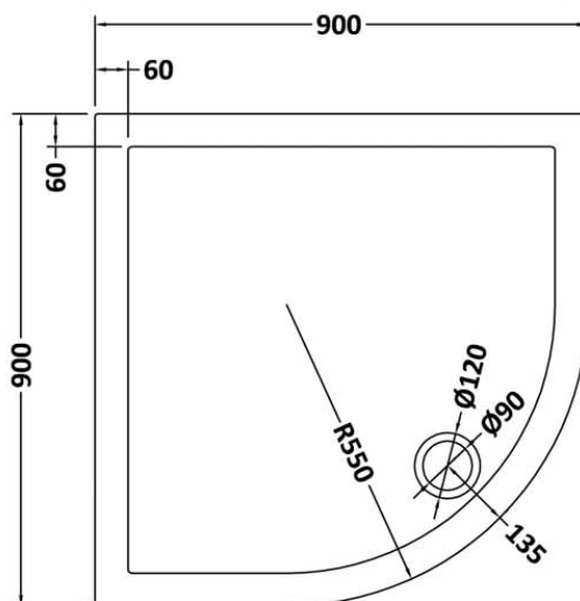
NTP106 - 900 x 900 QUADRANT TRAY
