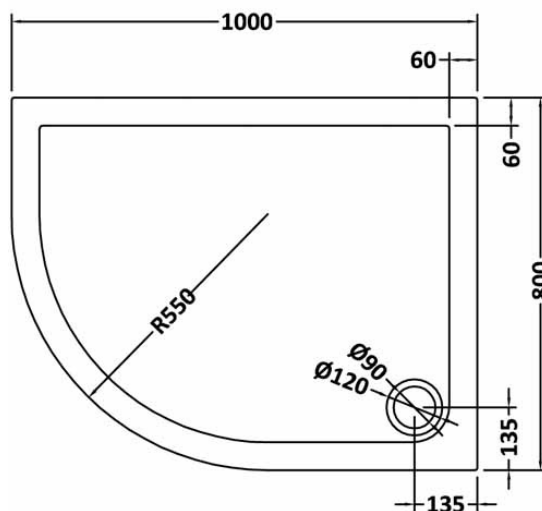
NTP108 - 1000 x 800 OFFSET QUADRANT TRAY LH
