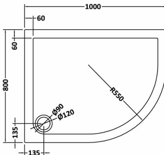
NTP109 - 1000 x 800 OFFSET QUADRANT TRAY RH
