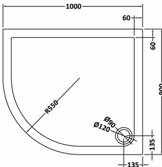
NTP110 - 1000 x 900 OFFSET QUADRANT TRAY LH
