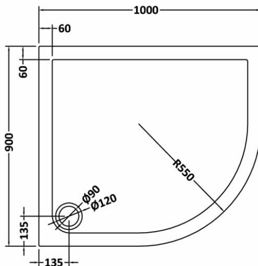
NTP111 - 1000 x 900 OFFSET QUADRANT TRAY RH
