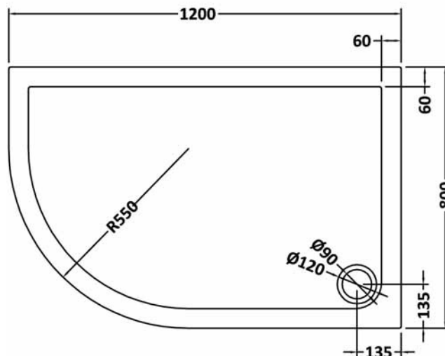
NTP112 - 1200 x 800 OFFSET QUADRANT TRAY LH
