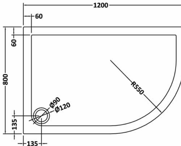
NTP113 - 1200 x 800 OFFSET QUADRANT TRAY RH
